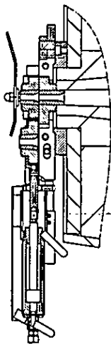
DETAIL 1 scale 1:5
